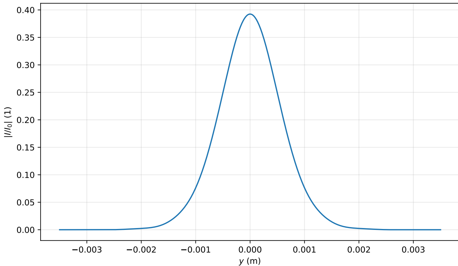
Intensity profile I(x=0, y, z=3.981)/I_0 , P_{in}=0.5P_{cr} , artificial time
